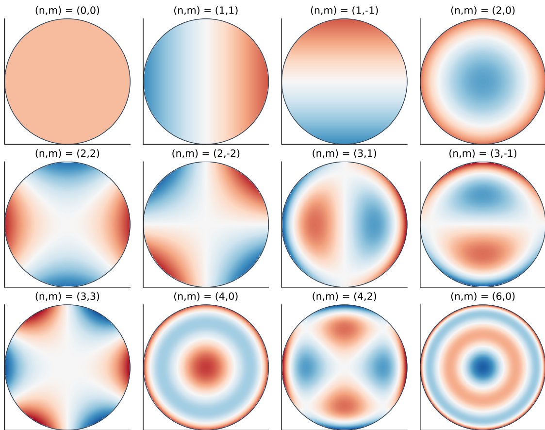
Figure 7.1: Original atlas of selected real, RMS-normalized modes. Red and blue indicate opposite OPD signs; the same colour scale is used throughout. The labels are (n,m) , not the paper's single-index coefficient numbers.
