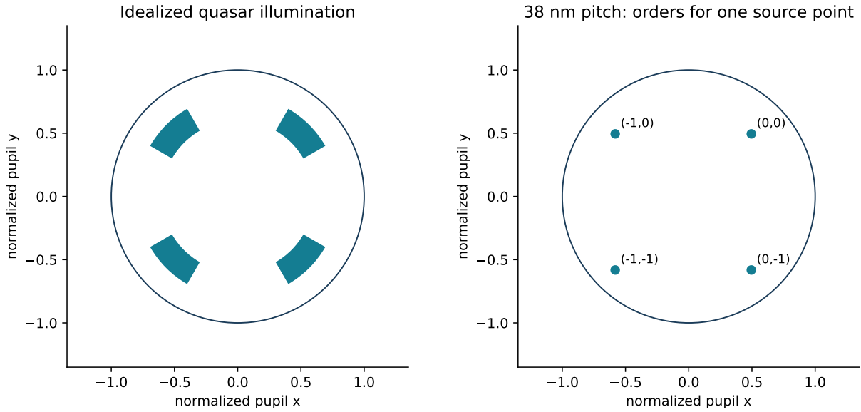
Figure 8.1: Original pupil diagrams. Left: an idealized four-sector quasar source. Right: shifted order locations for one diagonal source point and a 38 nm square pitch. Accepted orders can interfere to create a two-dimensional contact image. This is a thin-mask explanation, not a reproduction of the commercial simulator.
