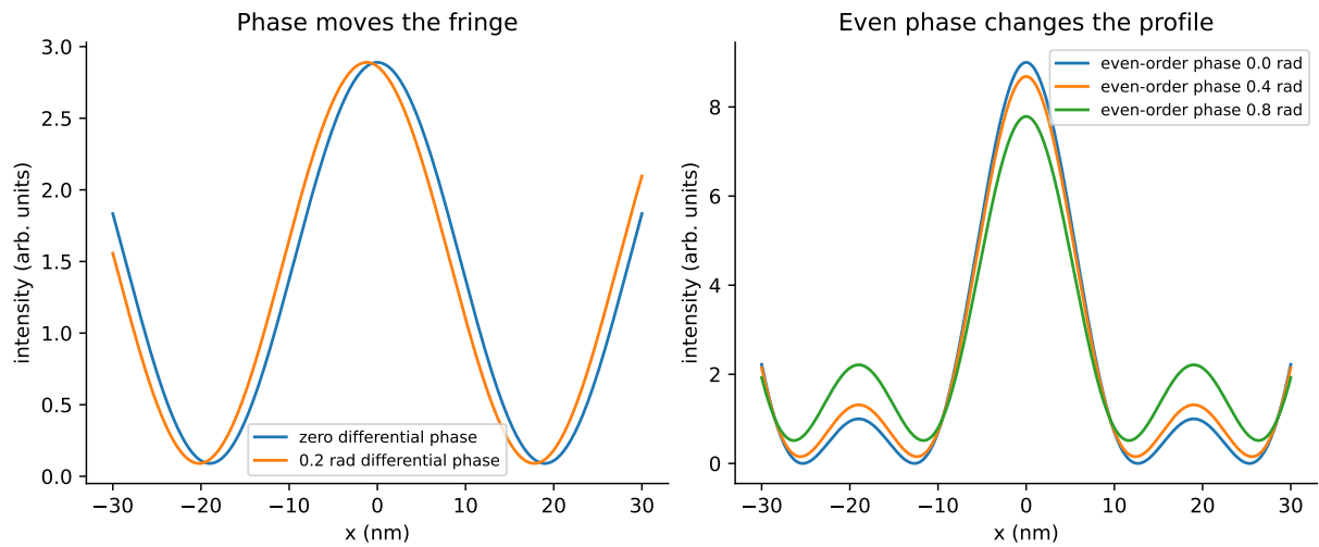
Figure 8.2: Exact teaching examples. A differential phase between two orders shifts fringes. A common phase on symmetric side orders changes an even intensity profile. A real contact combines many such interference terms and an incoherent source average.
