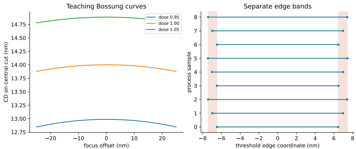
Figure 17.2: Left: teaching Bossung curves computed over a wider focus interval for illustration. Right: left and right edge positions for the nine stated focus-dose samples. Shaded regions show their individual process bands.
