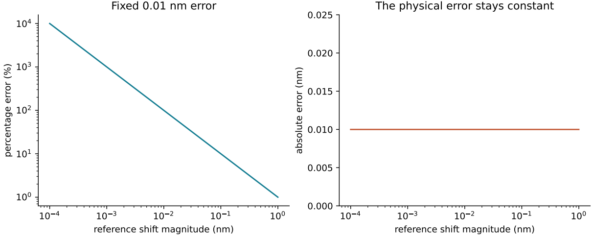
Figure 14.1: A fixed absolute error of 0.01 nm produces an arbitrarily large percentage as the reference shift approaches zero. The right panel shows that the physical error does not diverge.
